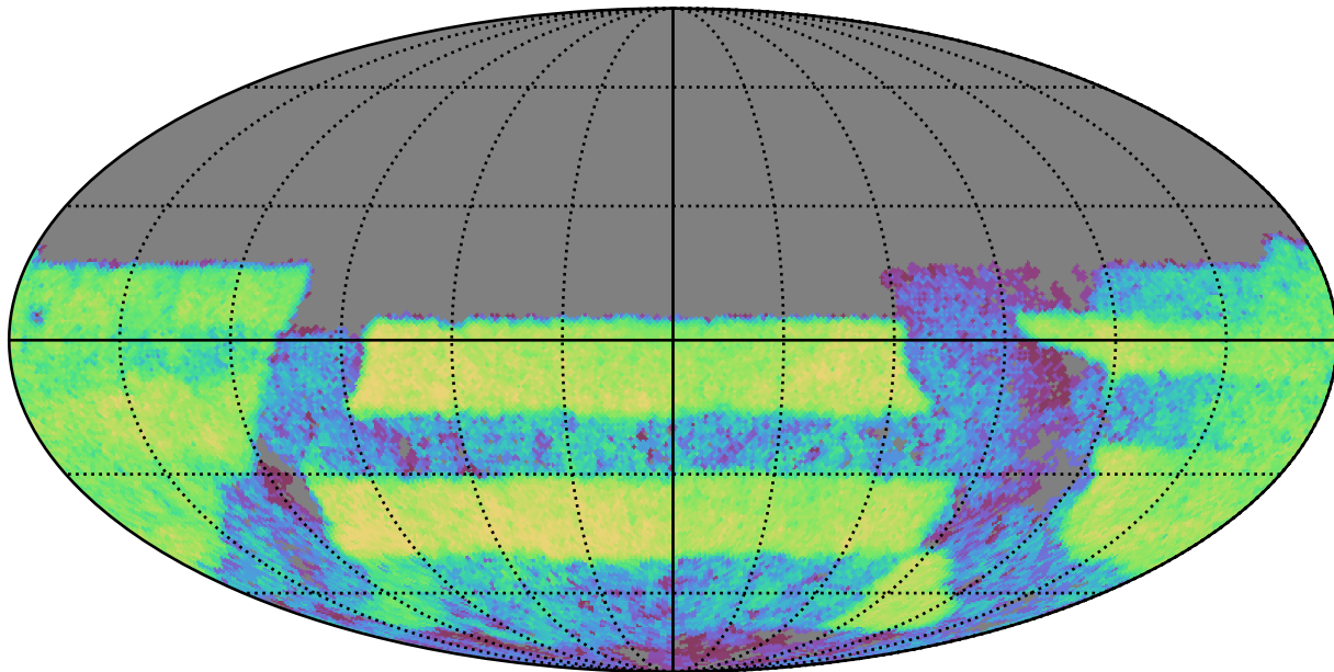
baseline_v2.1_10yrs Yr 3-4 y band: CoaddM5
