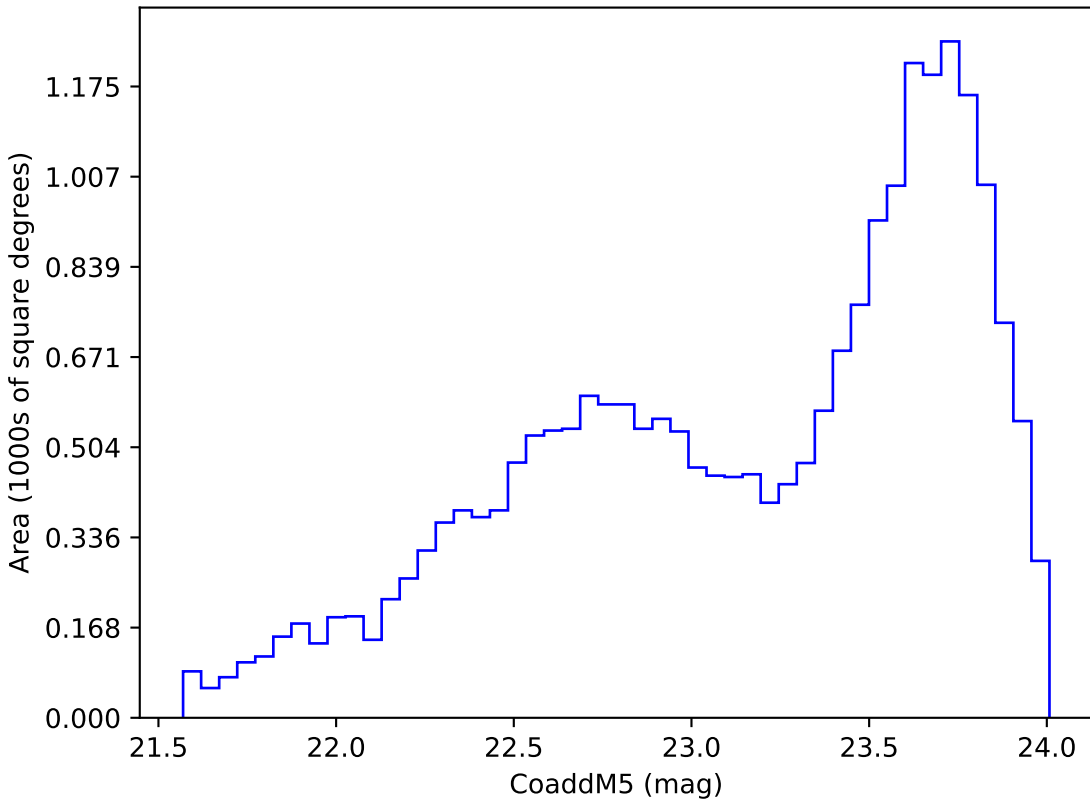
baseline_v2.1_10yrs Yr 3-4 y band: CoaddM5
