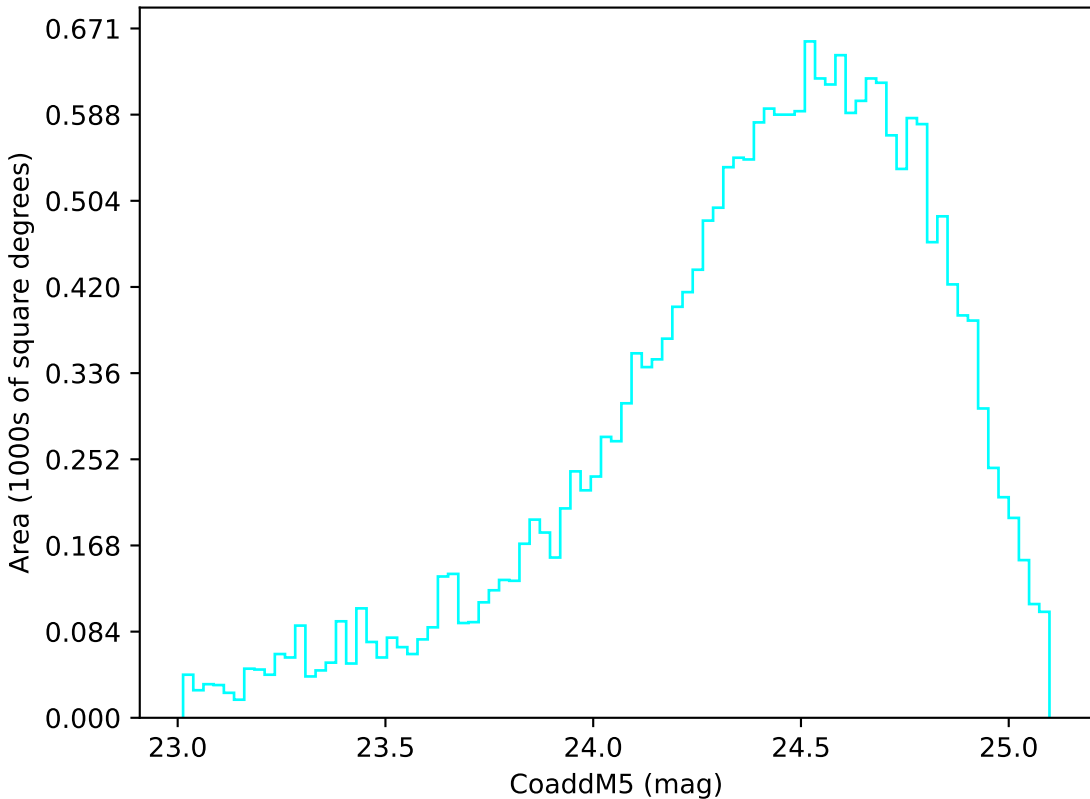
baseline_v2.1_10yrs Yr 3-4 u band: CoaddM5
