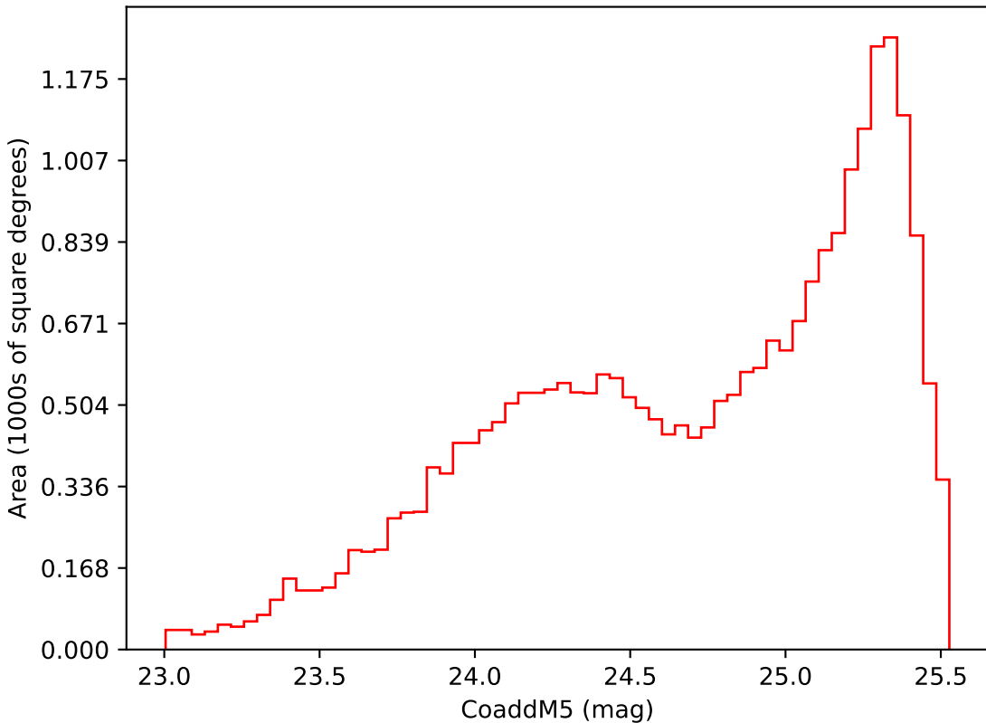
baseline_v2.1_10yrs Yr 3-4 i band: CoaddM5
