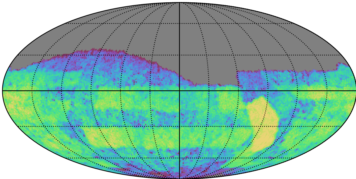
baseline_v2.1_10yrs Yr 3-4 g band: CoaddM5
