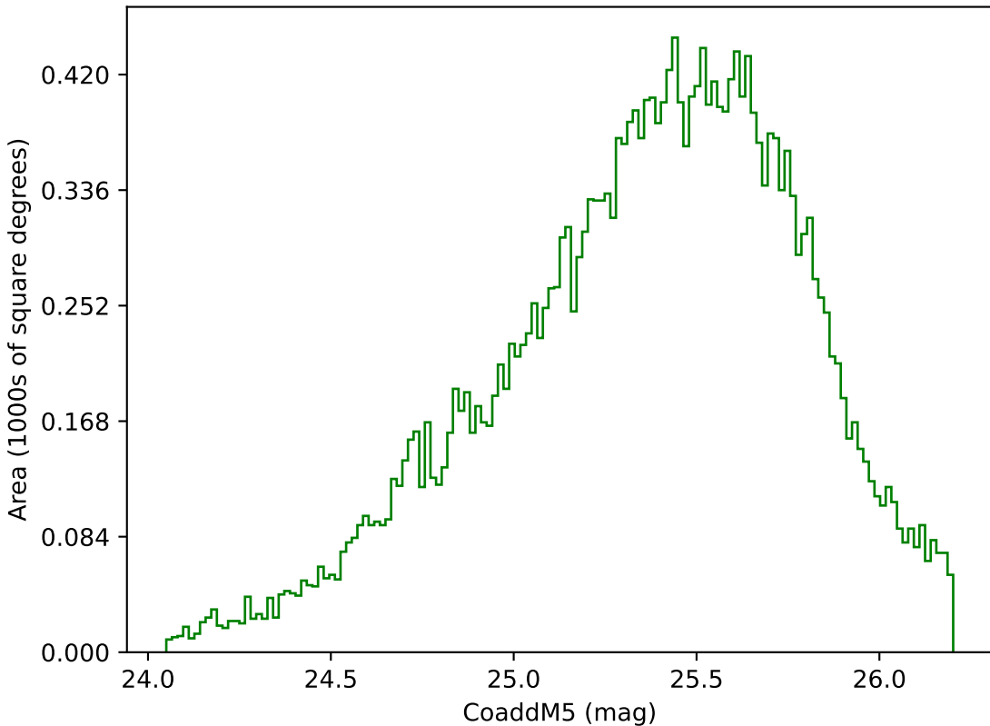
baseline_v2.1_10yrs Yr 3-4 g band: CoaddM5
