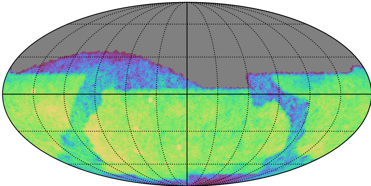
baseline_v2.1_10yrs Yr 1 z band: CoaddM5
