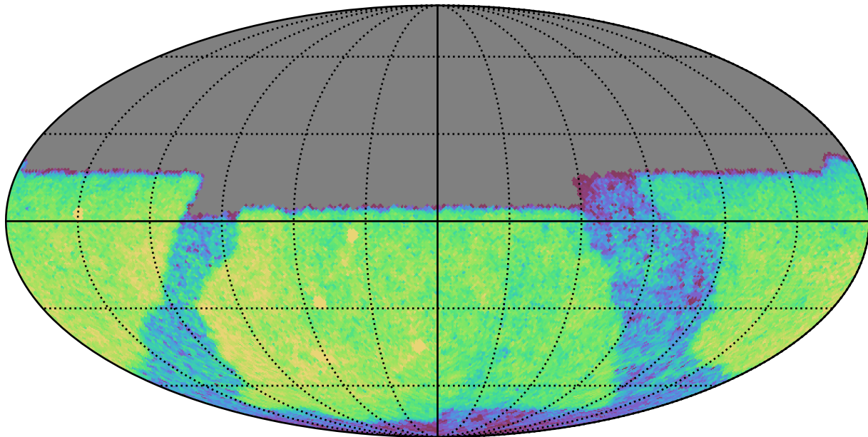
baseline_v2.1_10yrs Yr 1 y band: CoaddM5
