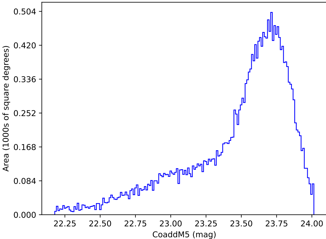
baseline_v2.1_10yrs Yr 1 y band: CoaddM5
