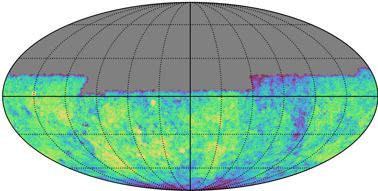
baseline_v2.1_10yrs Yr 1 u band: CoaddM5
