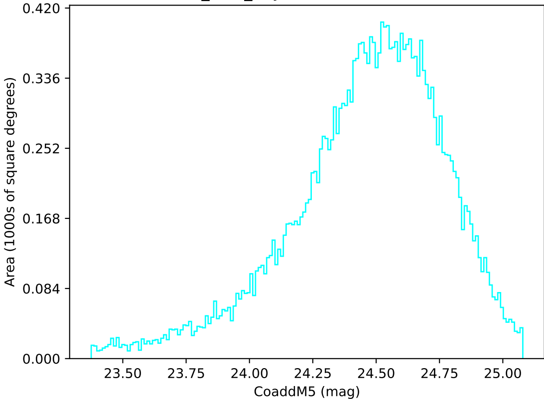
baseline_v2.1_10yrs Yr 1 u band: CoaddM5
