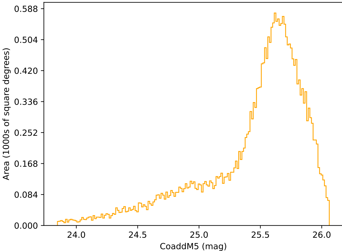
baseline_v2.1_10yrs Yr 1 r band: CoaddM5
