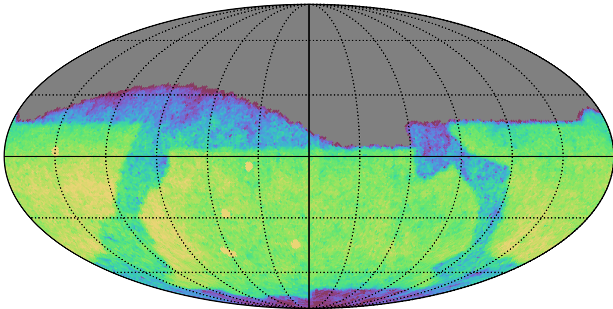
baseline_v2.1_10yrs Yr 1 i band: CoaddM5
