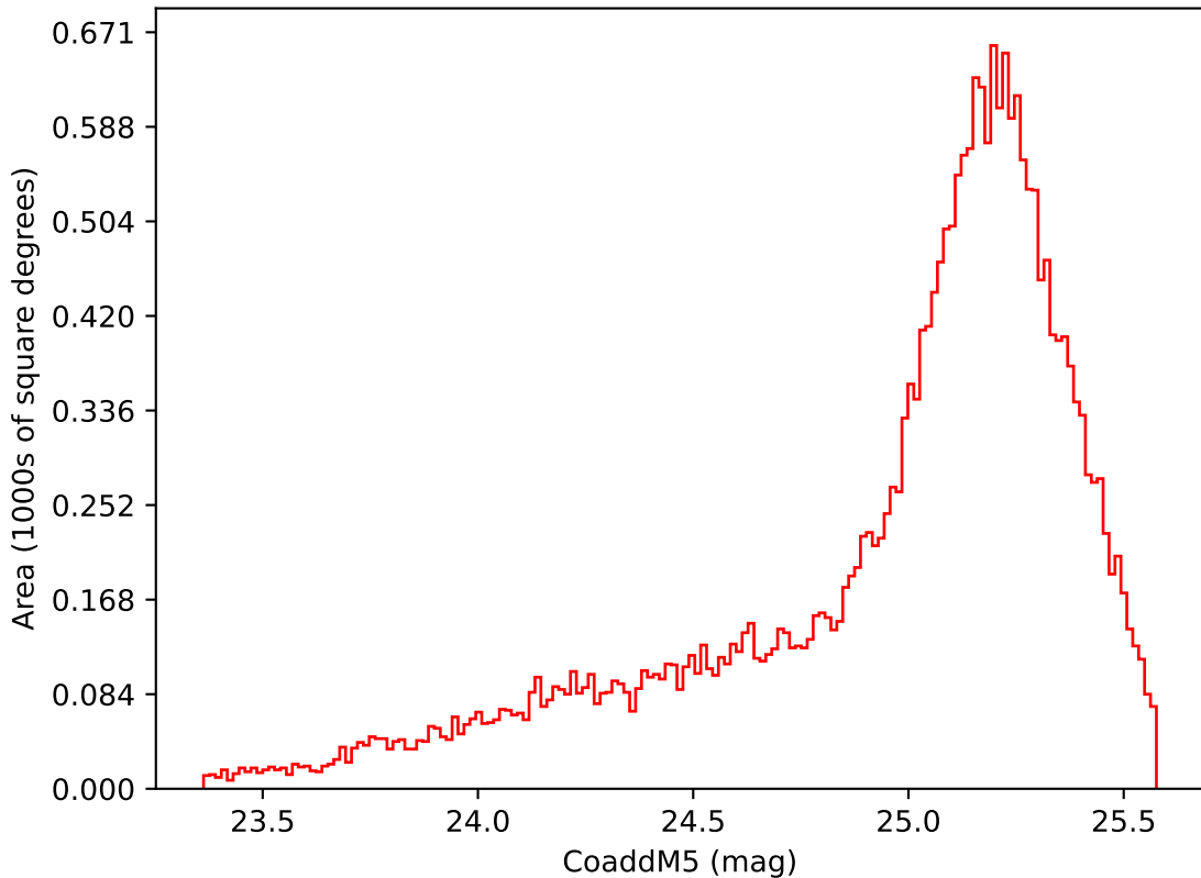
baseline_v2.1_10yrs Yr 1 i band: CoaddM5
