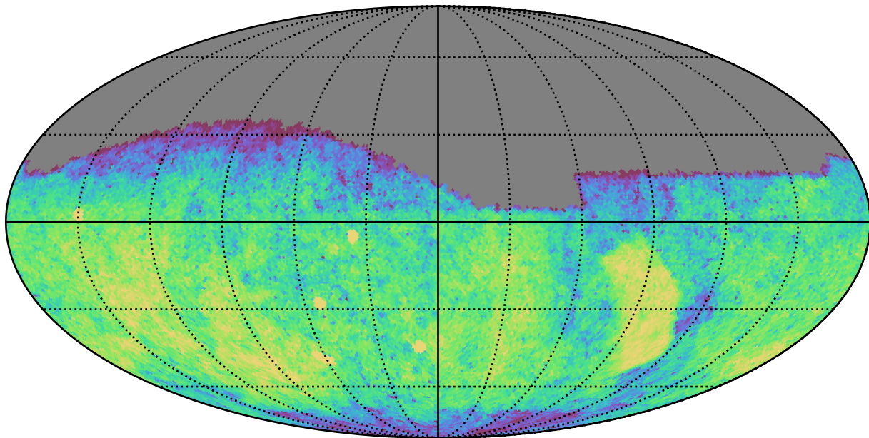
baseline_v2.1_10yrs Yr 1 g band: CoaddM5
