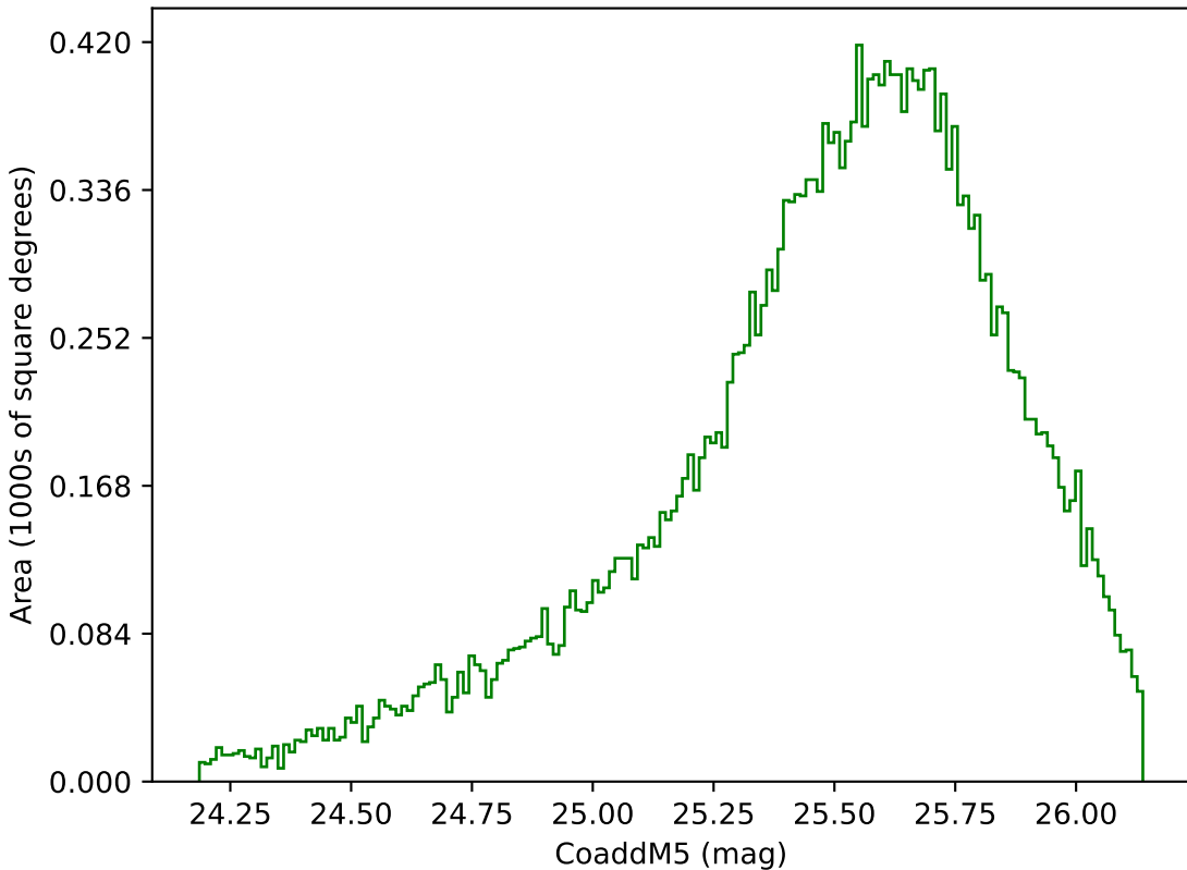
baseline_v2.1_10yrs Yr 1 g band: CoaddM5
