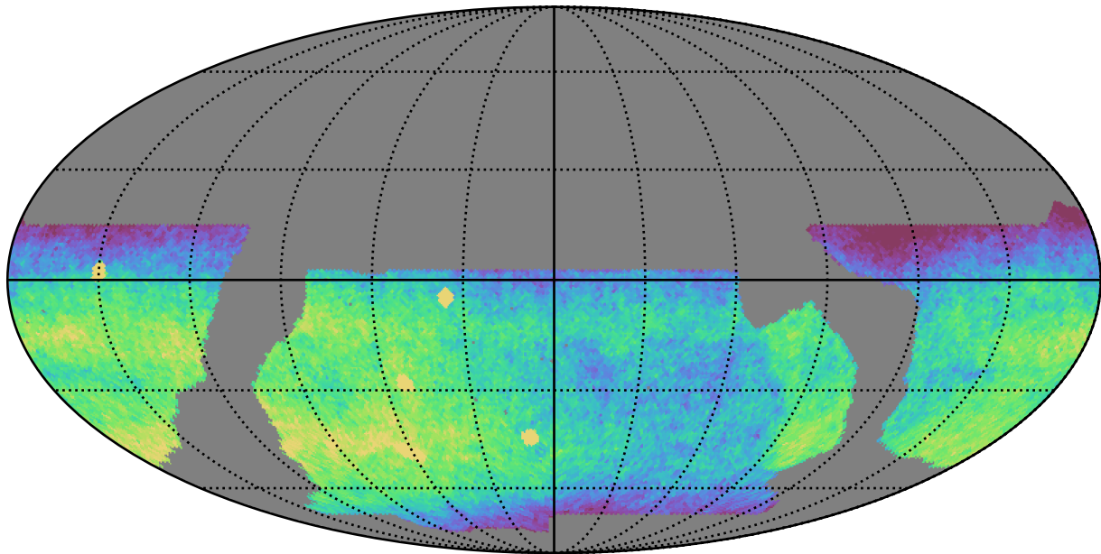
baseline_v2.1_10yrs WFD z band: CoaddM5
