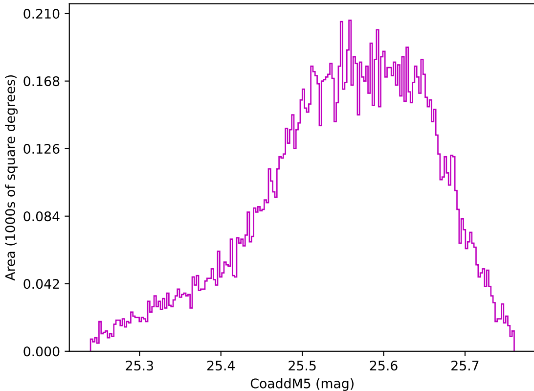
baseline_v2.1_10yrs WFD z band: CoaddM5
