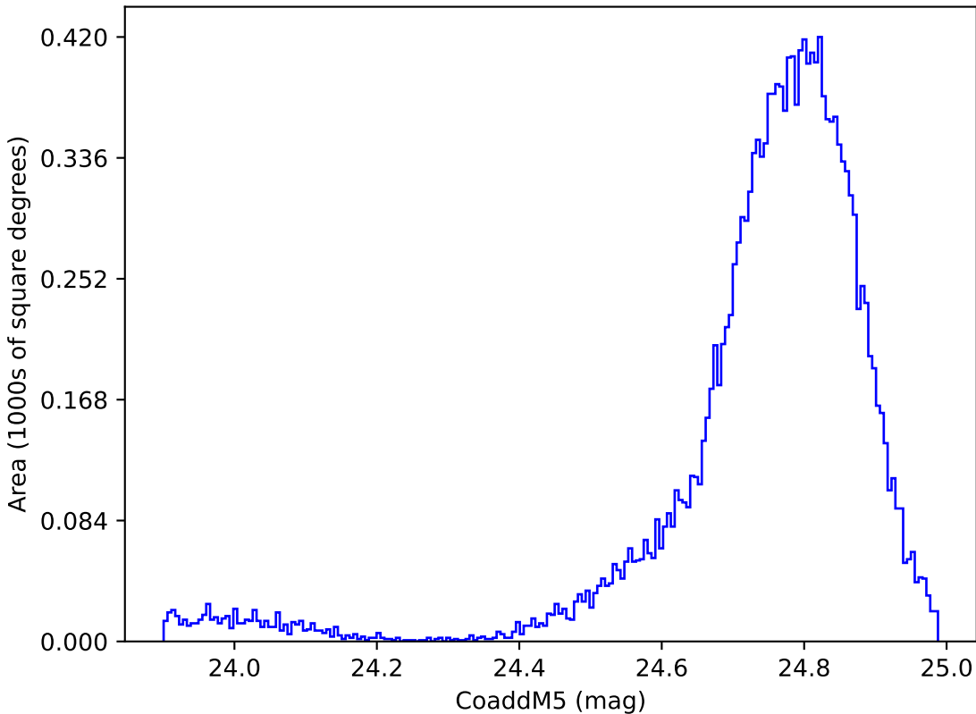
baseline_v2.1_10yrs WFD y band: CoaddM5
