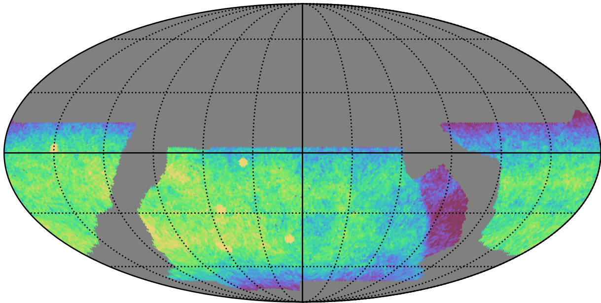
baseline_v2.1_10yrs WFD u band: CoaddM5
