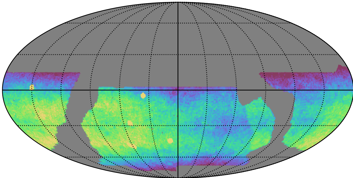
baseline_v2.1_10yrs WFD r band: CoaddM5
