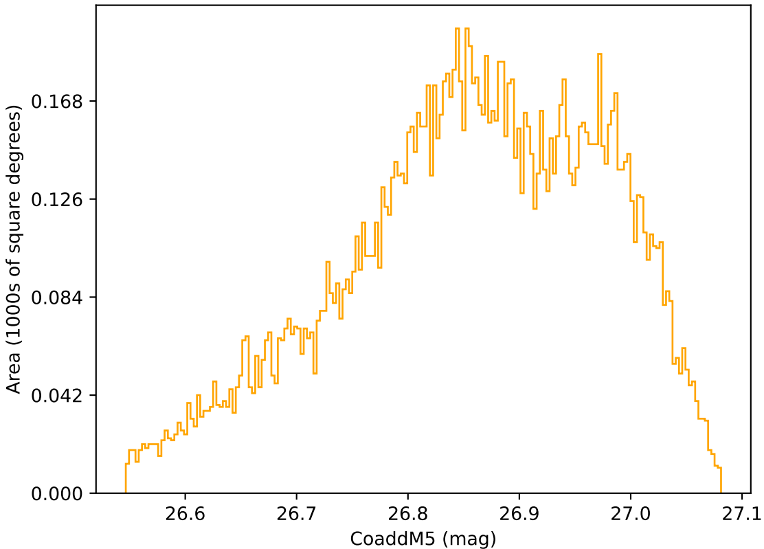
baseline_v2.1_10yrs WFD r band: CoaddM5
