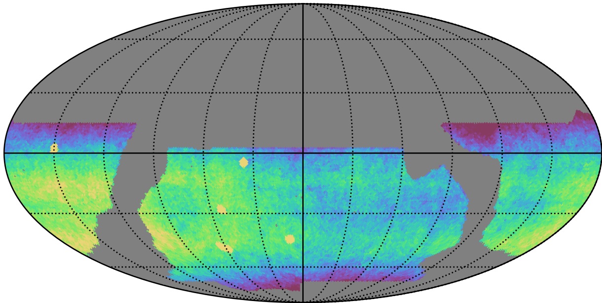
baseline_v2.1_10yrs WFD i band: CoaddM5
