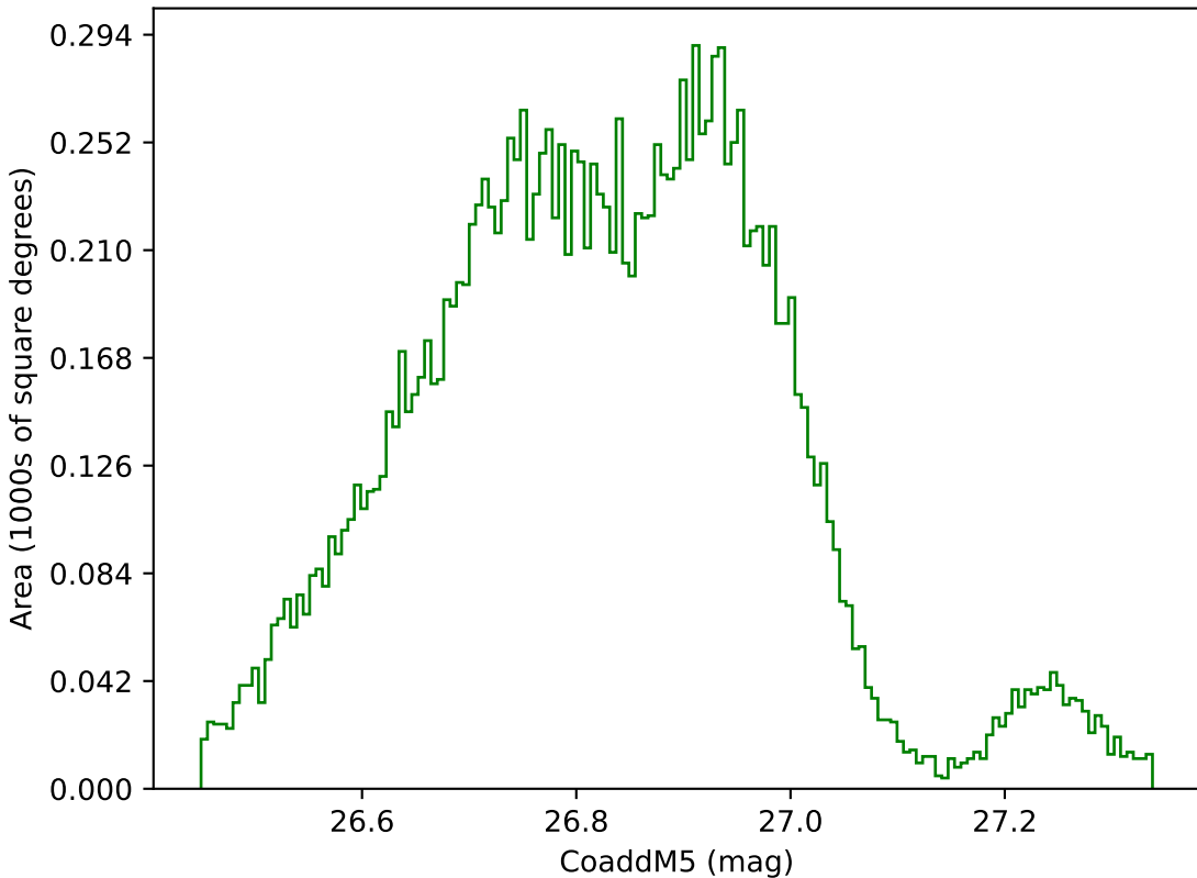
baseline_v2.1_10yrs WFD g band: CoaddM5
