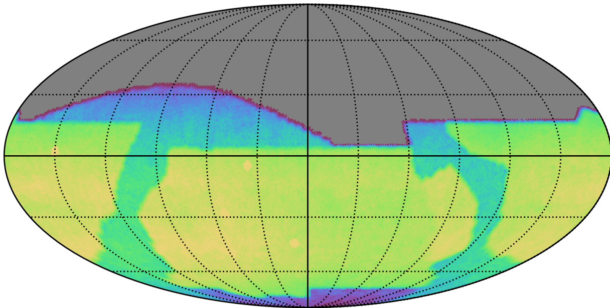
baseline_v2.1_10yrs All sky z band: CoaddM5
