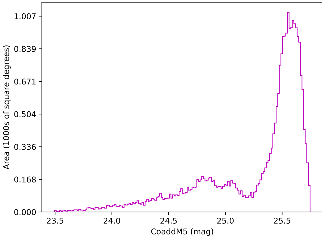
baseline_v2.1_10yrs All sky z band: CoaddM5
