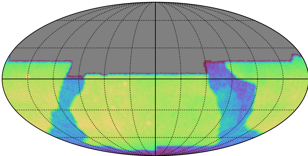
baseline_v2.1_10yrs All sky y band: CoaddM5
