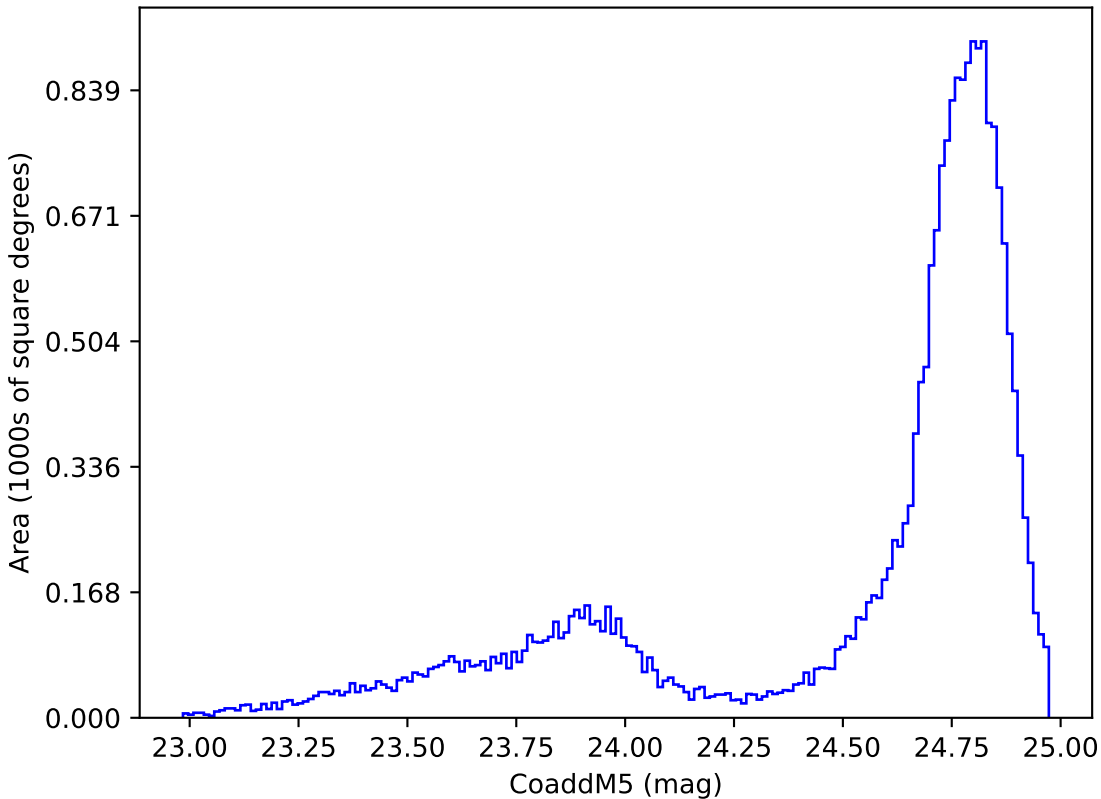
baseline_v2.1_10yrs All sky y band: CoaddM5
