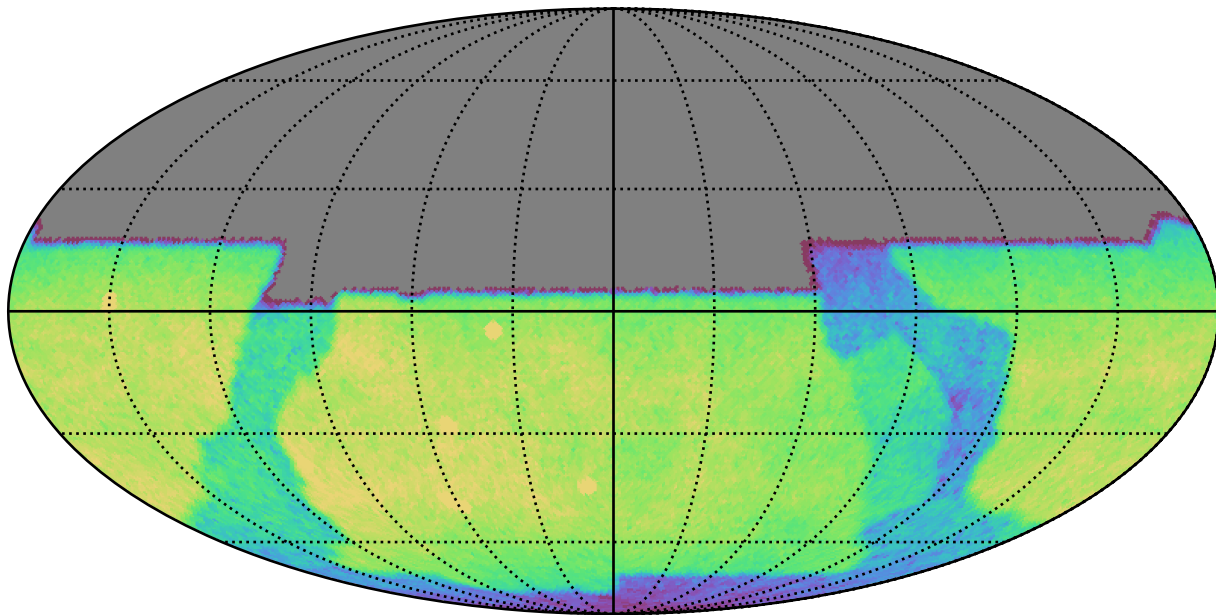
baseline_v2.1_10yrs All sky u band: CoaddM5
