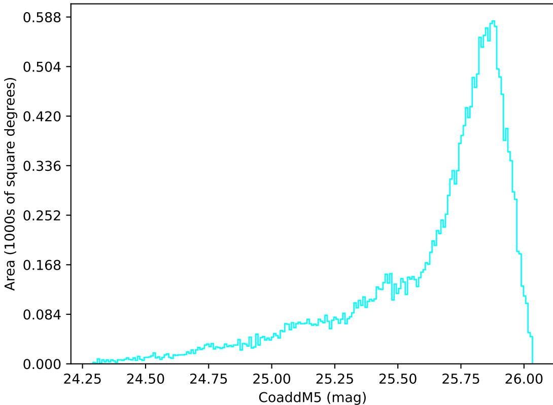
baseline_v2.1_10yrs All sky u band: CoaddM5
