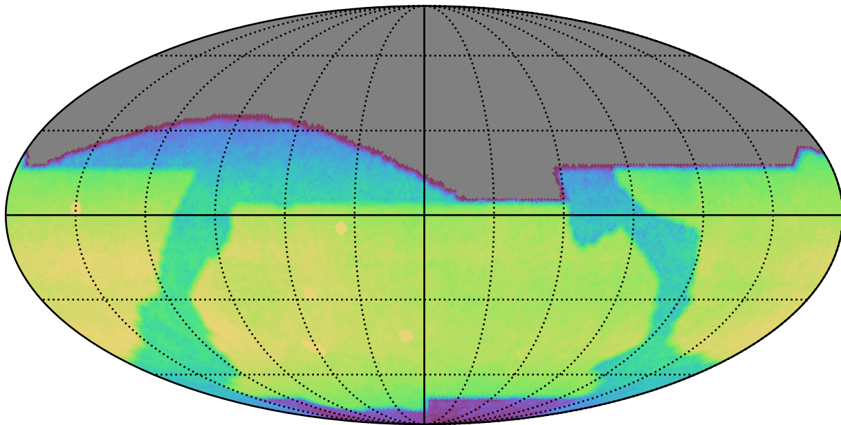
baseline_v2.1_10yrs All sky i band: CoaddM5
