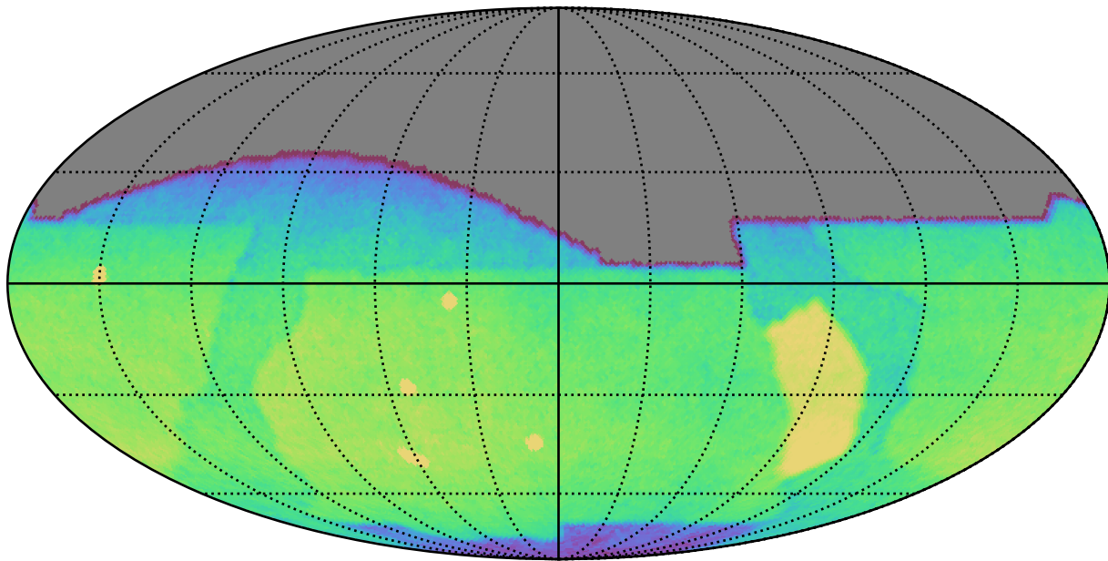
baseline_v2.1_10yrs All sky g band: CoaddM5
