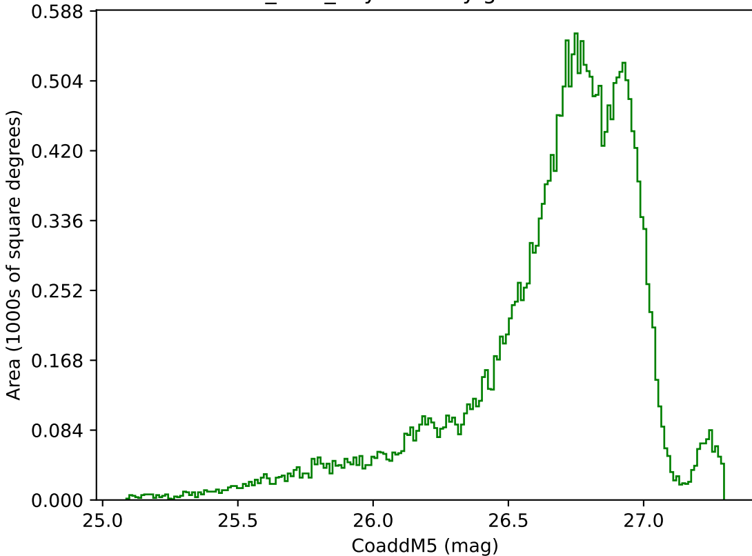
baseline_v2.1_10yrs All sky g band: CoaddM5
