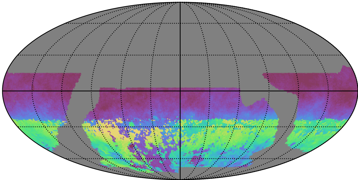
baseline_v2.1_10yrs WFD z band: AngleRms rotSkyPos
