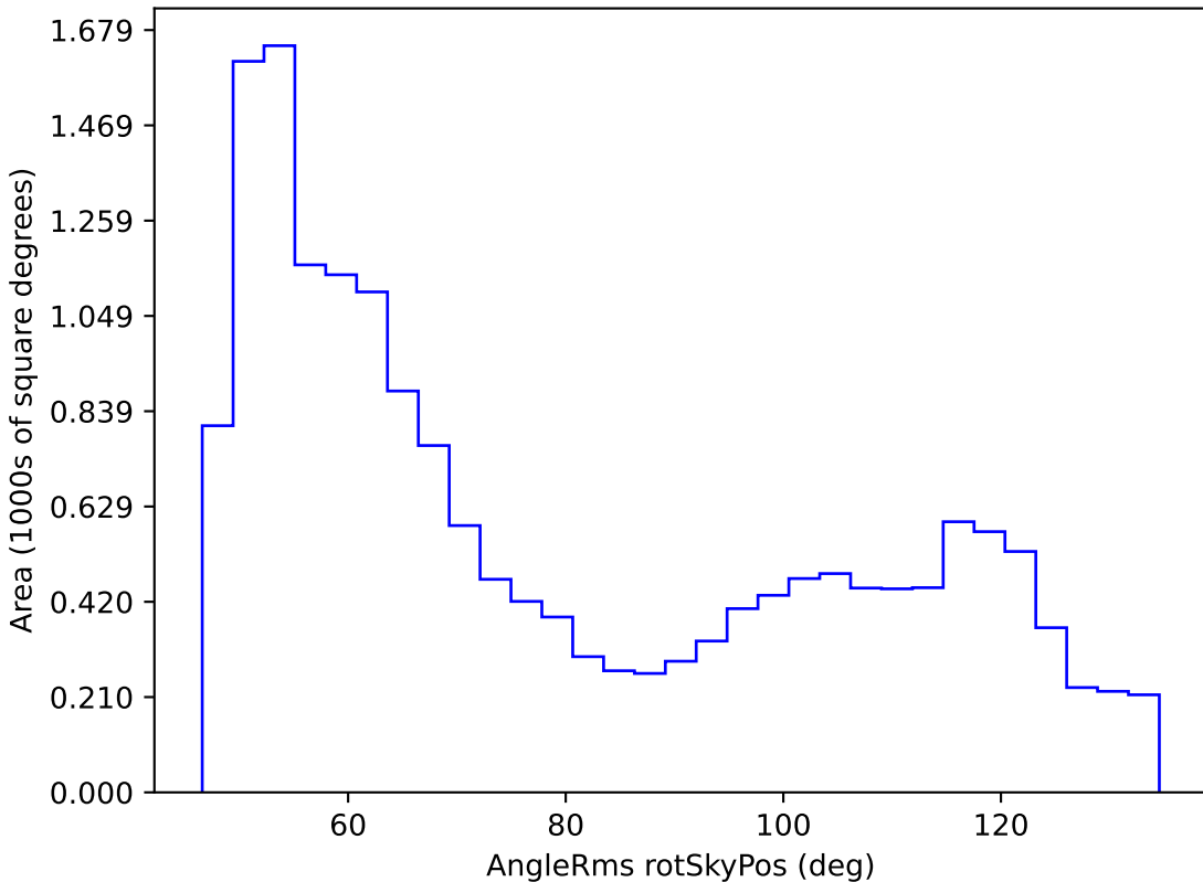
baseline_v2.1_10yrs WFD z band: AngleRms rotSkyPos
