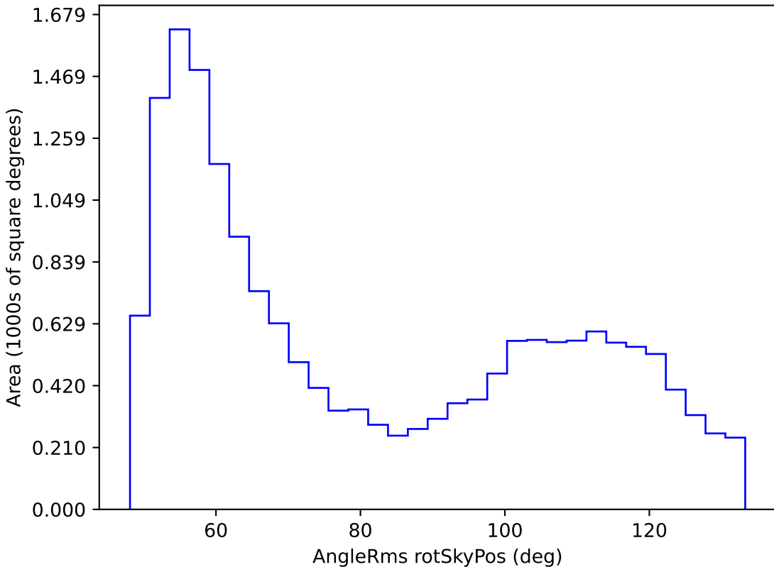
baseline_v2.1_10yrs WFD y band: AngleRms rotSkyPos
