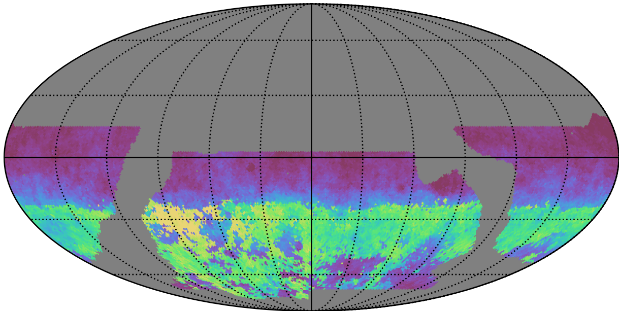
baseline_v2.1_10yrs WFD u band: AngleRms rotSkyPos
