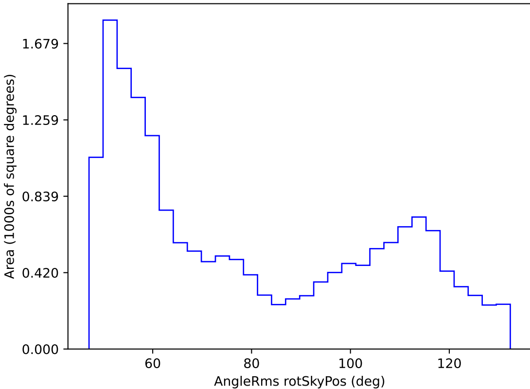
baseline_v2.1_10yrs WFD r band: AngleRms rotSkyPos
