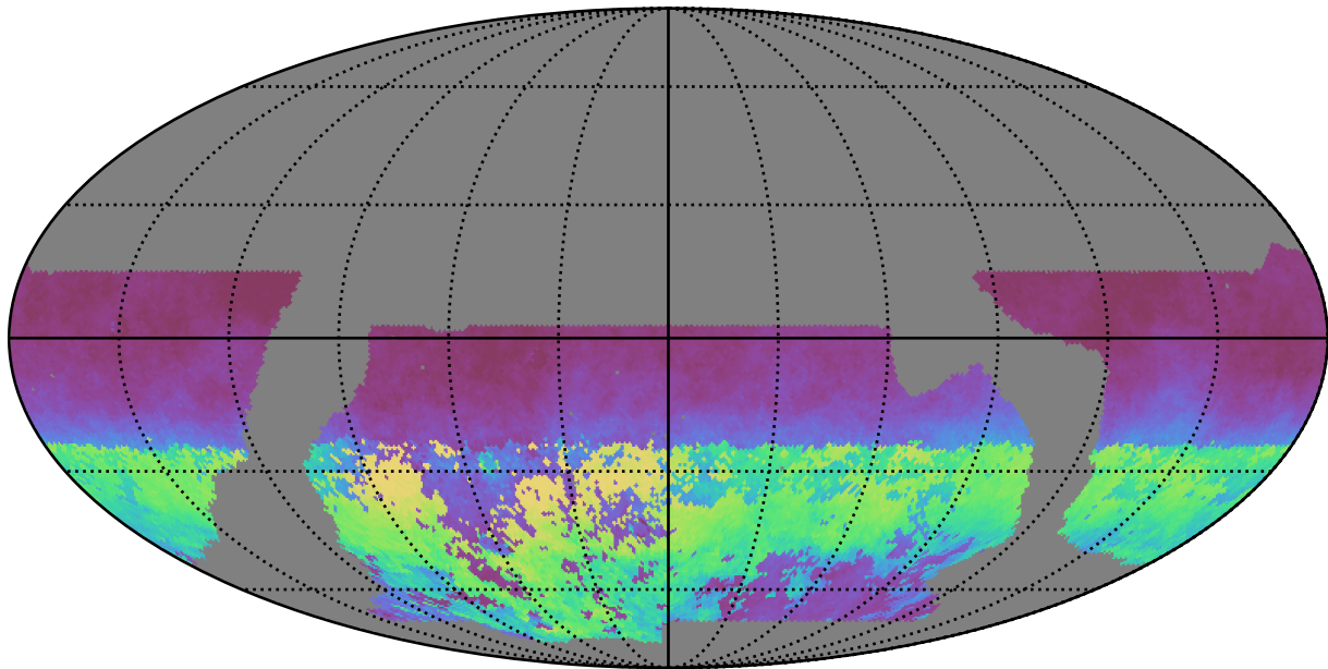
baseline_v2.1_10yrs WFD i band: AngleRms rotSkyPos
