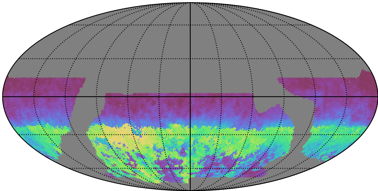
baseline_v2.1_10yrs WFD g band: AngleRms rotSkyPos
