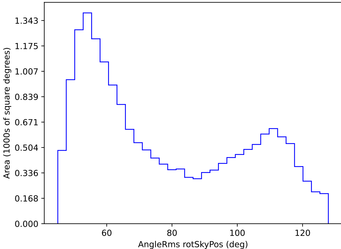
baseline_v2.1_10yrs WFD g band: AngleRms rotSkyPos
