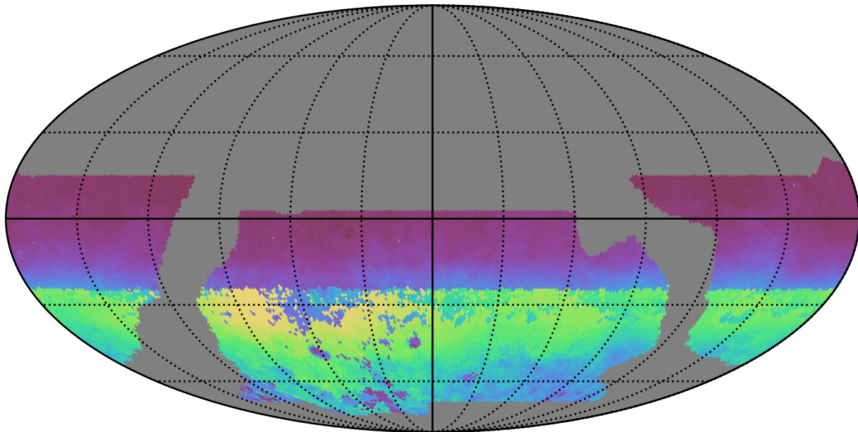
baseline_v2.1_10yrs WFD all bands: AngleRms rotSkyPos
