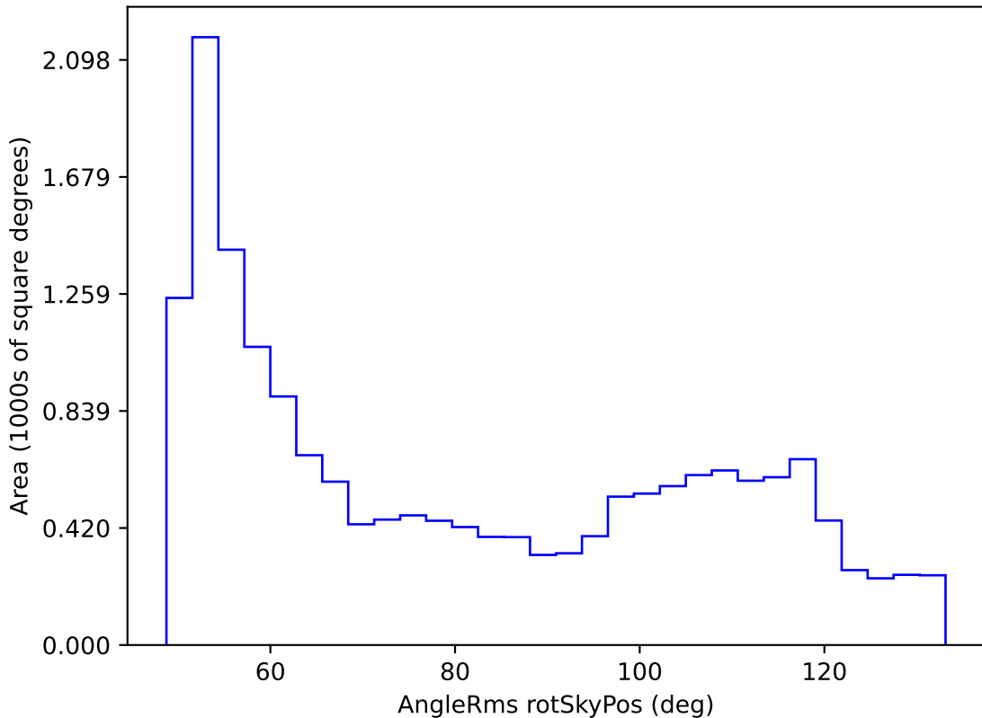
baseline_v2.1_10yrs WFD all bands: AngleRms rotSkyPos
