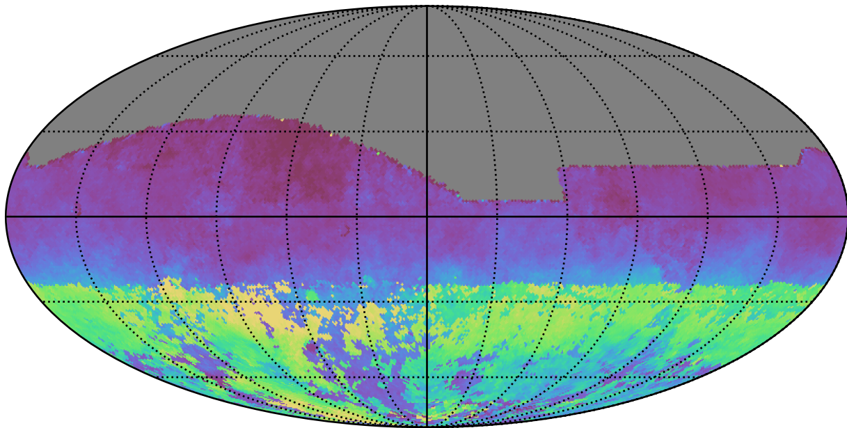
baseline_v2.1_10yrs All sky z band: AngleRms rotSkyPos
