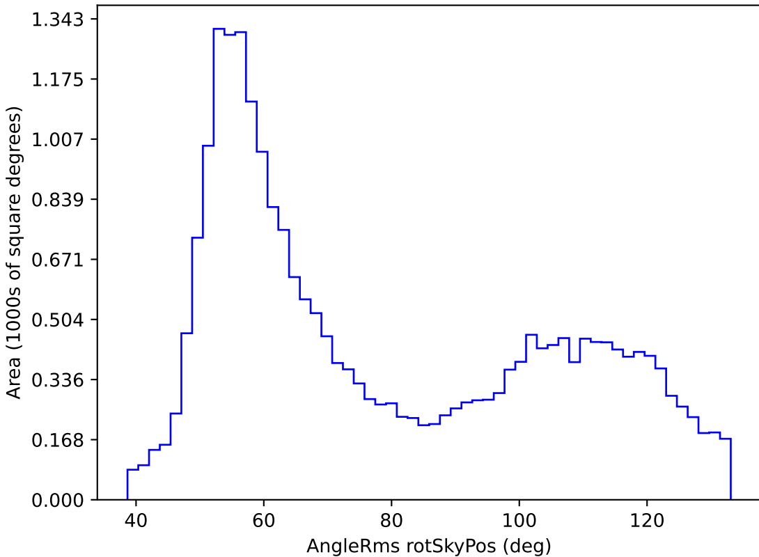
baseline_v2.1_10yrs All sky y band: AngleRms rotSkyPos
