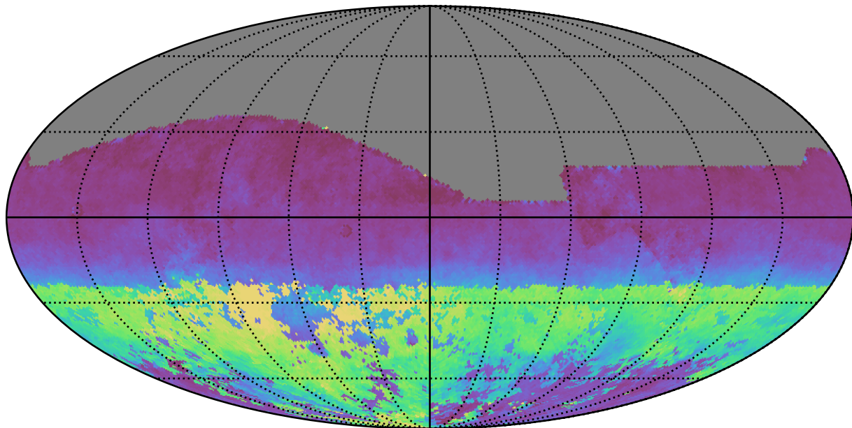
baseline_v2.1_10yrs All sky r band: AngleRms rotSkyPos
