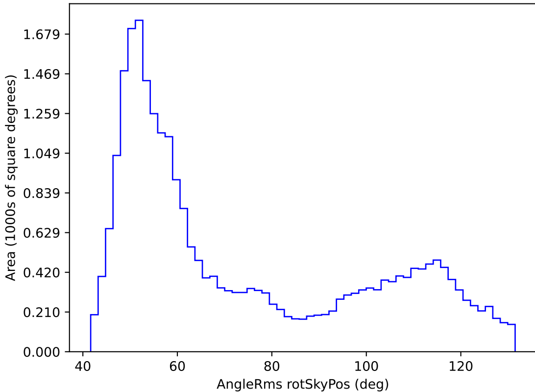
baseline_v2.1_10yrs All sky r band: AngleRms rotSkyPos
