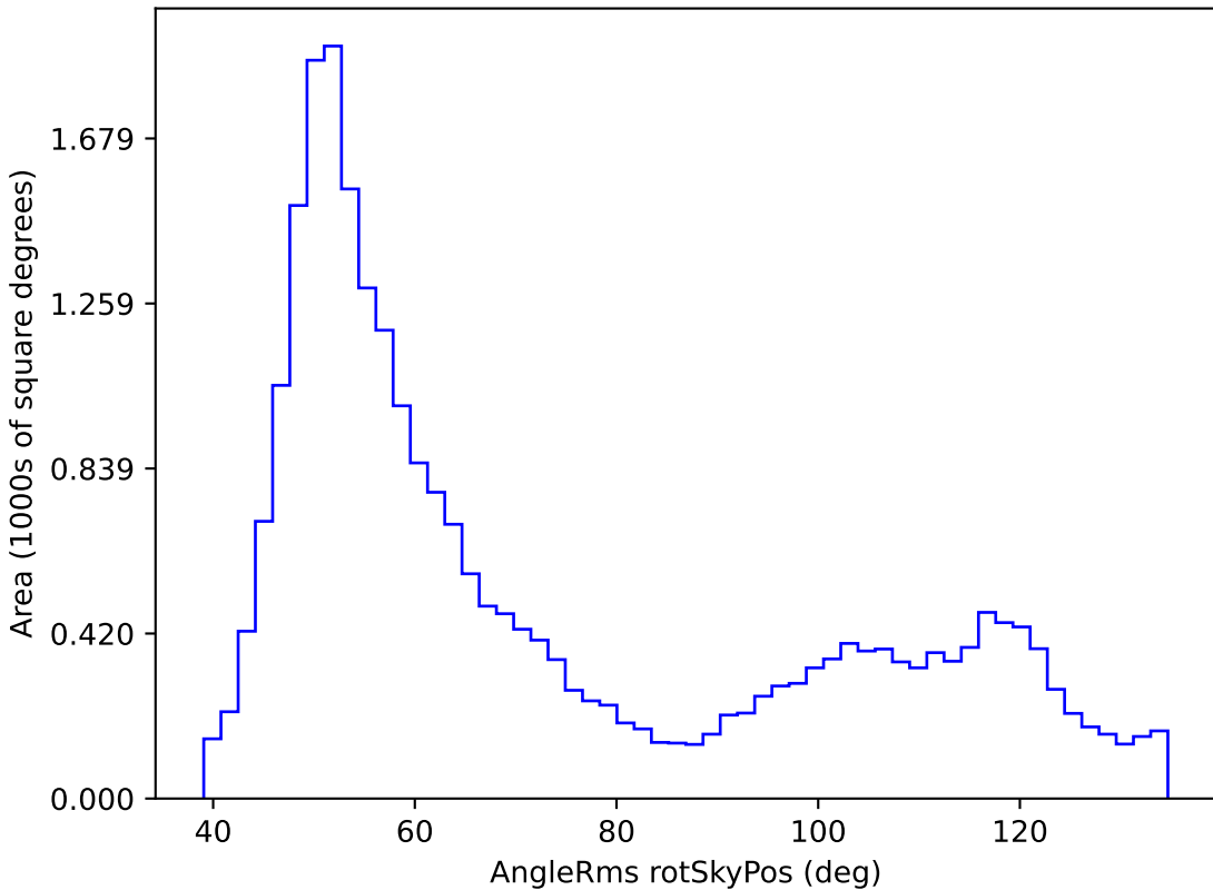
baseline_v2.1_10yrs All sky i band: AngleRms rotSkyPos
