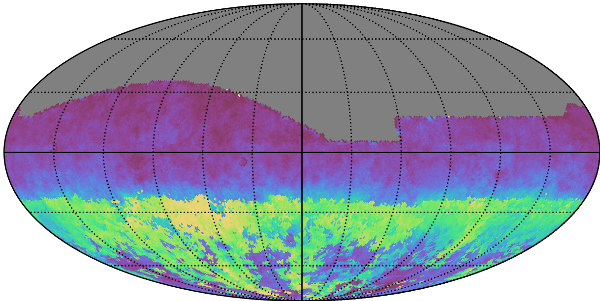
baseline_v2.1_10yrs All sky g band: AngleRms rotSkyPos
