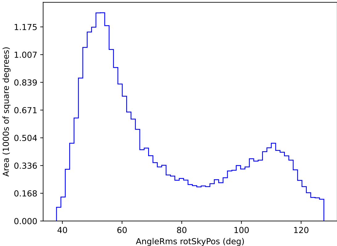
baseline_v2.1_10yrs All sky g band: AngleRms rotSkyPos
